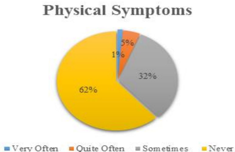
Graph 1. Histogram of Physical Symptoms Indicator Data About Stress Symptoms
