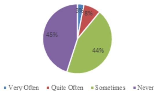
Graph 3. Histogram of Behavioral Symptom Indicator Data About Stress Symptoms
