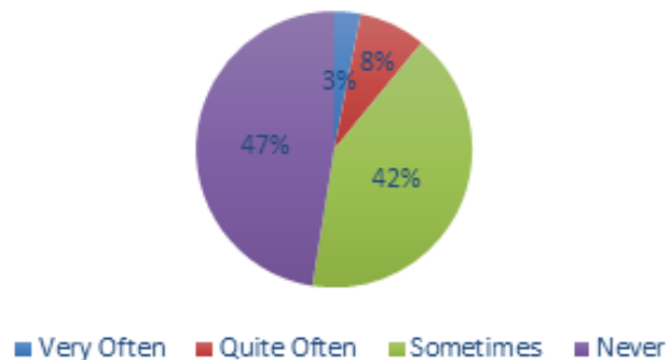
Graph 2. Histogram of Psychological Symptom Indicator Data About Stress Symptoms
